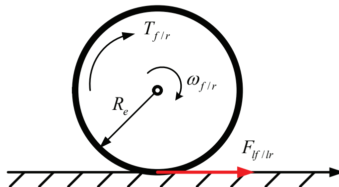
Figure 3. Wheel dynamics model.
